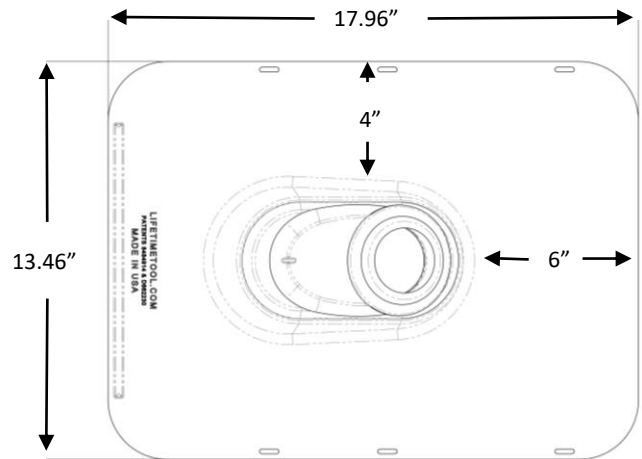
Plate Size: 1 ¼" ; 1 ½" & 2"
